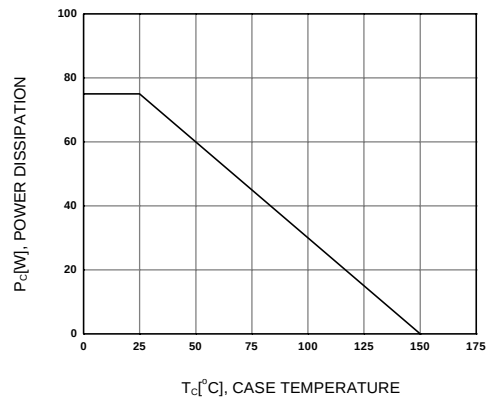
Figure 12. Power Derating
