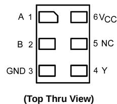
Pad Assignment for MicroPak
