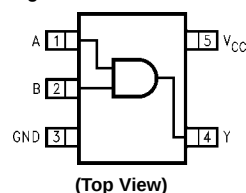
Pad Assignment for MicroPak
