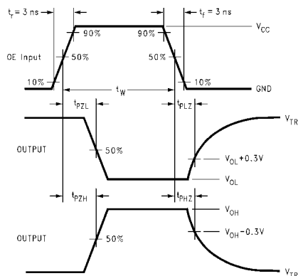
FIGURE 3. AC Waveforms
