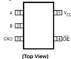
Pad Assignments for MicroPak
