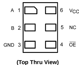
Pad Assignments for MicroPak
