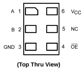
Pad Assignments for MicroPak
