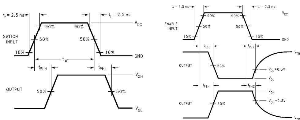
FIGURE 2. AC Waveforms
