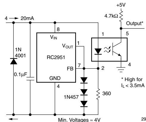
Figure 11. Open Circuit Detector for 4mA to 20mA Current Loop
