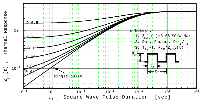
Fig 11. Thermal Response
