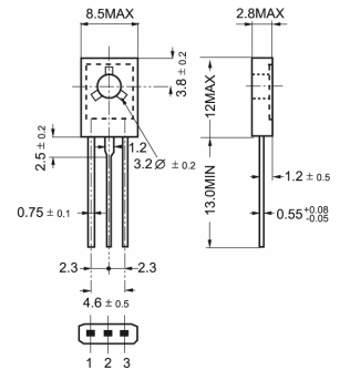
TO-126
