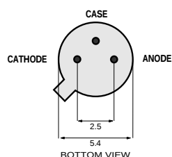
TO-46 Package With Lens
