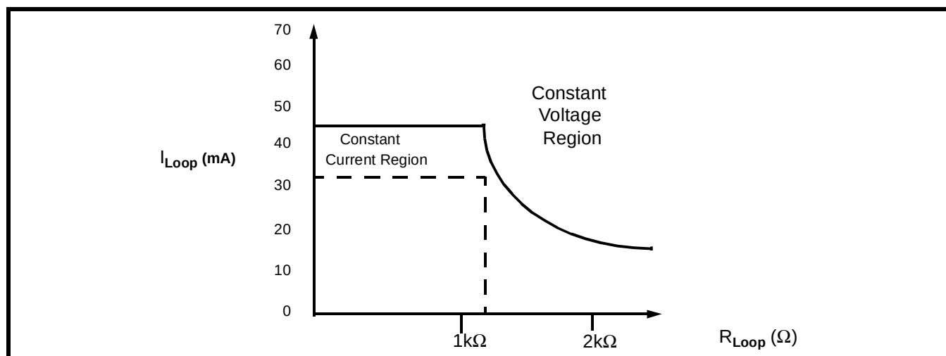
Graph 1 - I_{Loop}/R_{Loop} Characteristics
