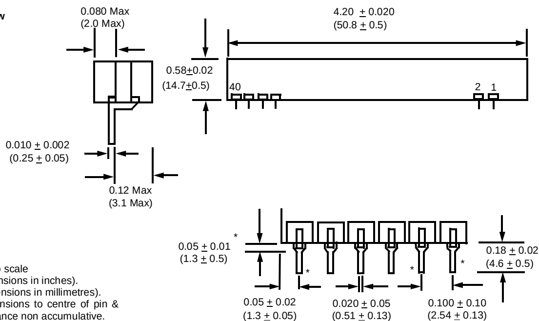
Figure 10 - Mechanical Data
