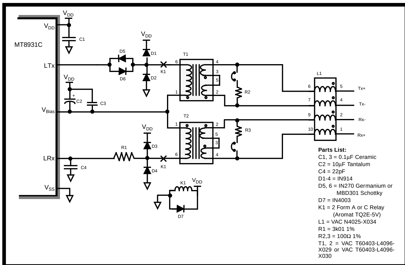
Figure 22 - ETS 300-012 NT & TE Line Interface for VAC X029 or X030
