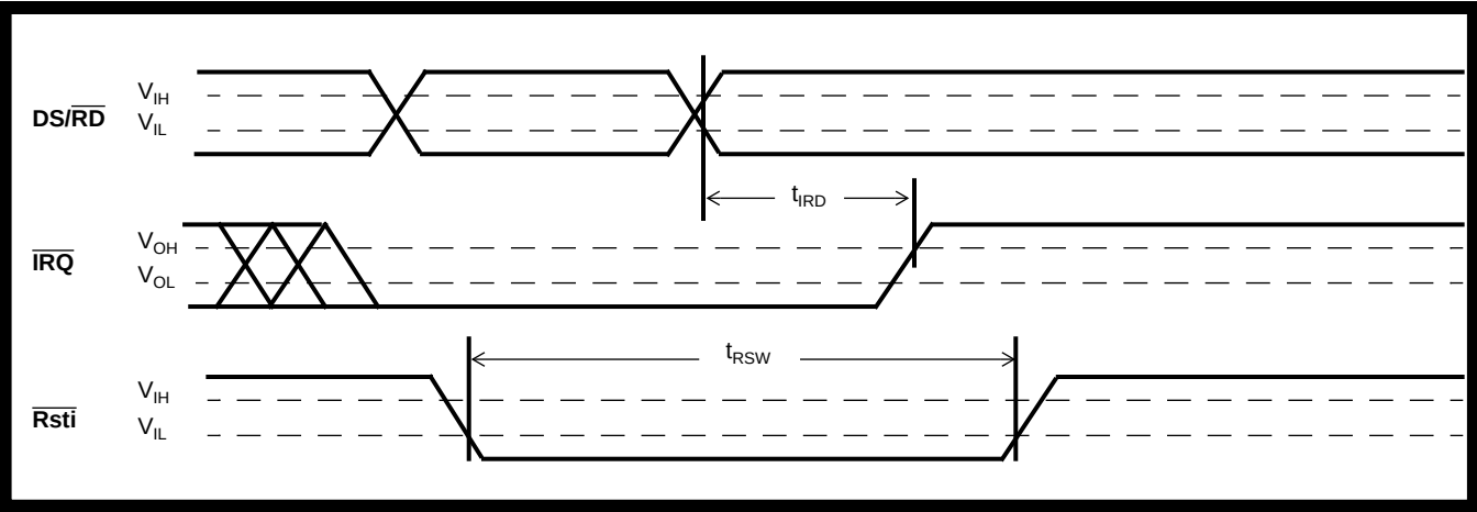
Figure 27 - \overline{\text{INT}} & \overline{\text{Rsti}} Timing
