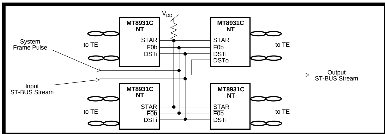
Figure 14 - NT in Star Configuration
