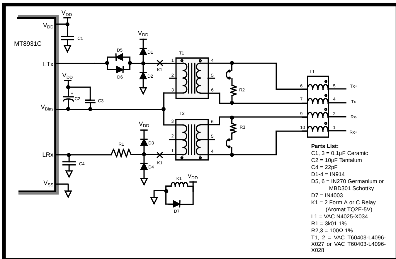
Figure 21 - ETS 300-012 NT & TE Line Interface for VAC X027 or X028
