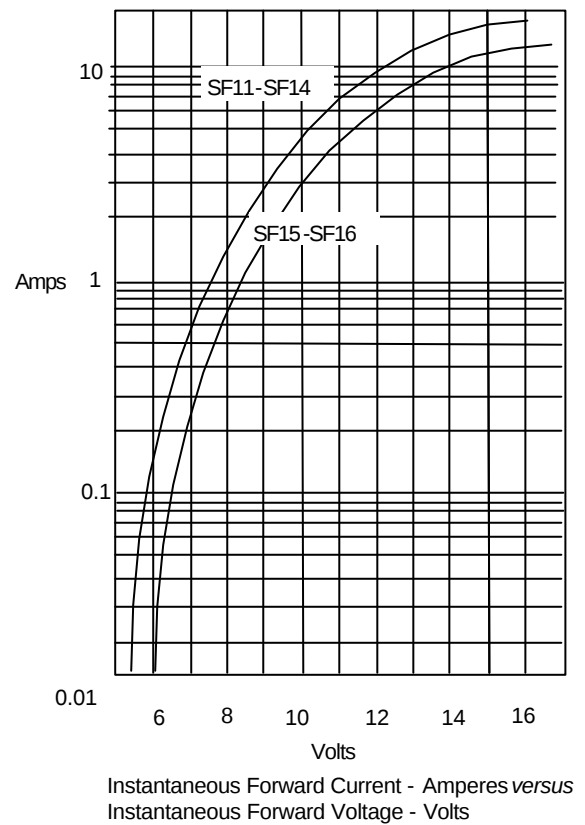
Figure 2 Typical Forward Characteristics
