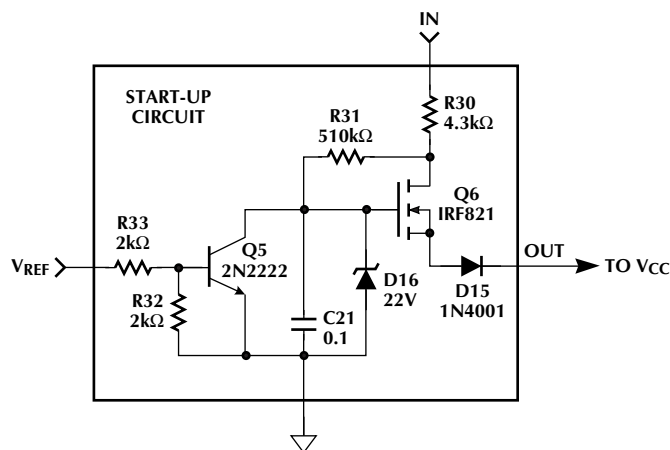
Figure 13. Start-Up Circuit
