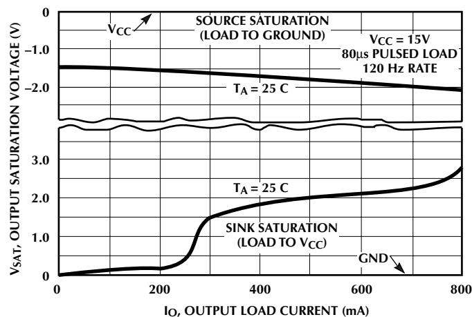
Figure 3. Output Saturation Voltage vs. Output Current
