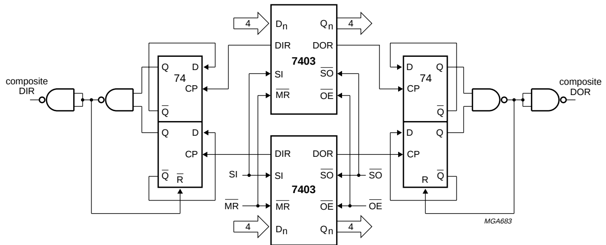
Fig.19 Expanded FIFO for increased word length.
