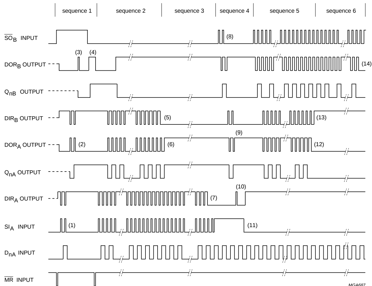
Fig.23 Waveforms showing the functionality and intercommunication between two FIFOs (refer to Fig.18).
