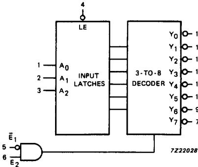
Fig.2 Logic symbol.
