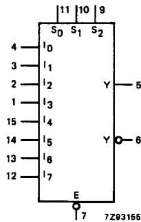
Fig.2 Logic symbol.
