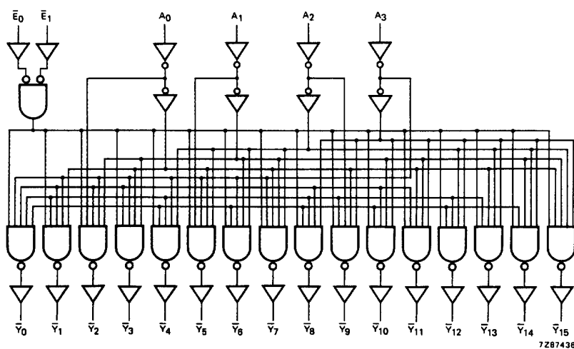
Fig.5 Logic diagram.
