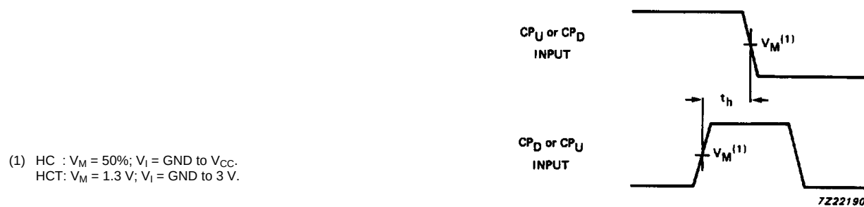
Fig.13 Waveforms showing the CP_U to CP_D or CP_D to CP_U hold times.
