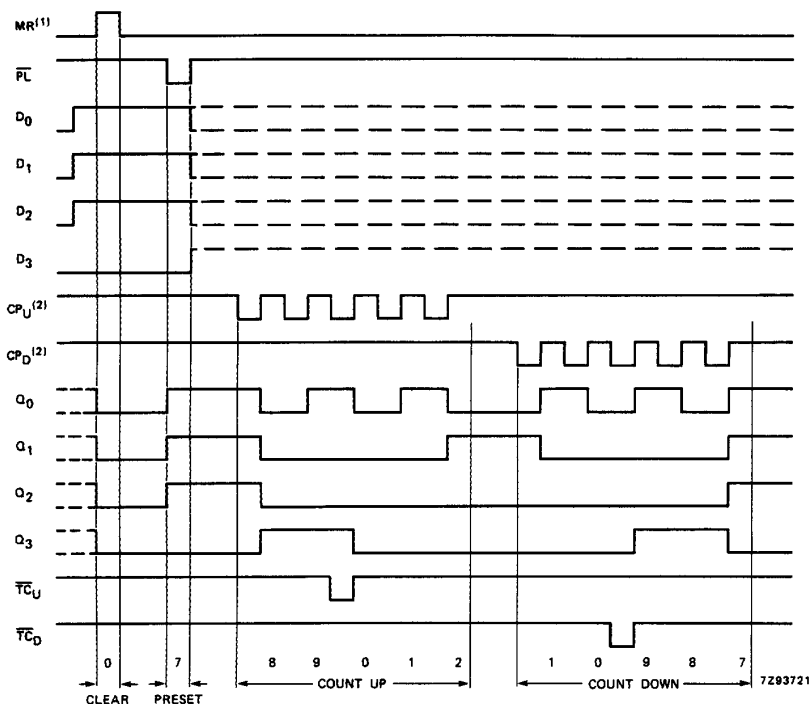
Fig.5 Typical clear, load and count sequence.
