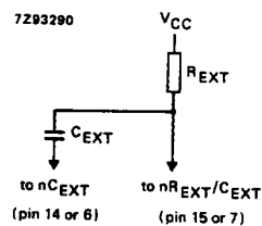
Fig.6 Timing component connections.
