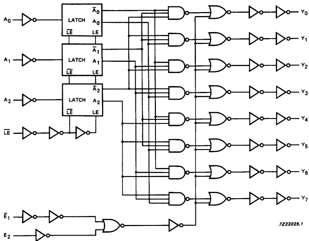
Fig.5 Logic diagram.
