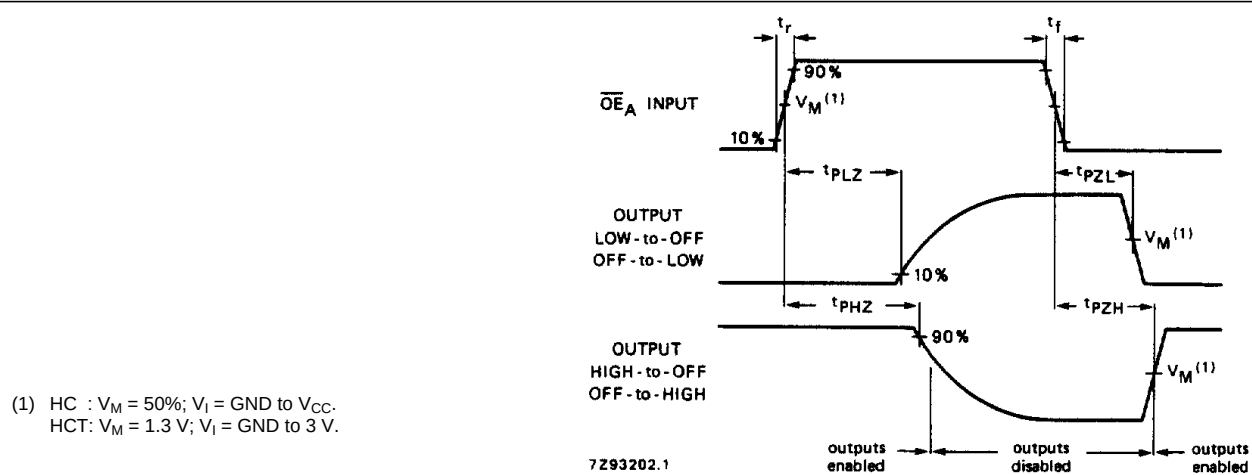
Fig.7 Waveforms showing the 3-state enable and disable times for input OE_A .
