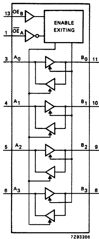
Fig.4 Functional diagram.
