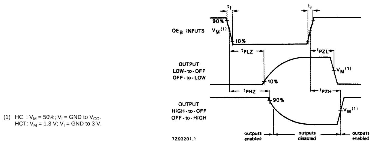
Fig.6 Waveforms showing the 3-state enable and disable times for input OE_B .
