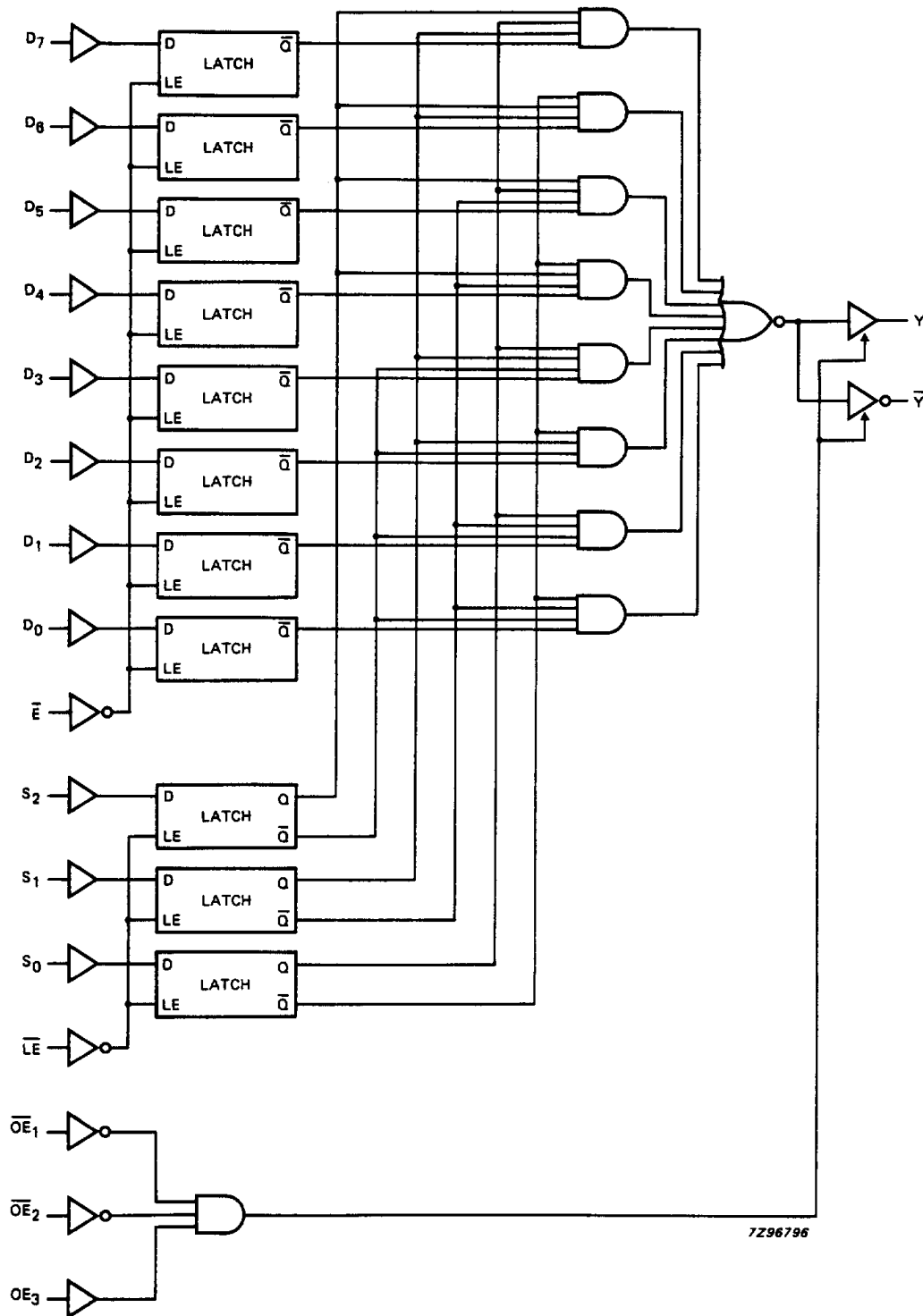
Fig.5 Logic diagram.
