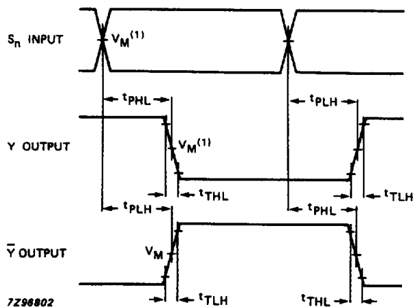
Fig.8 Waveforms showing the select input ( S_n ) to output ( Y, \bar{Y} ) propagation delays and the output transition times ( \bar{LE} = \text{LOW} ).
