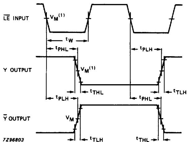
Fig.9 Waveforms showing the address latch enable input ( \bar{LE} ) pulse width, the address latch enable input to output ( Y, \bar{Y} ) propagation delays and the output transition times.
