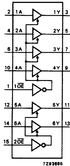
Fig.4 Functional diagram.
