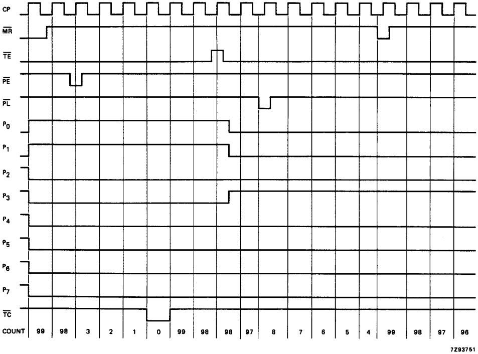
Fig.6 Timing diagram.
