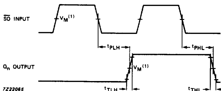
Fig.14 Waveforms showing \overline{SO} input to Q_n output propagation delays and output transition time.
