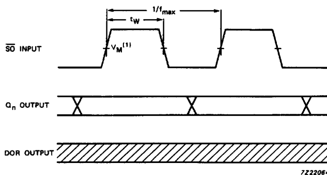
Fig.12 Waveforms showing \overline{SO} minimum pulse width and maximum pulse frequency, in high-speed shift-out burst mode.
