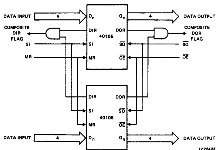
Fig.17 Expanded FIFO for increased word length; 16 words \times 8 bits.
