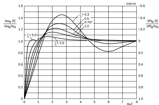
Fig.33 Type 2, second order frequency step response.
