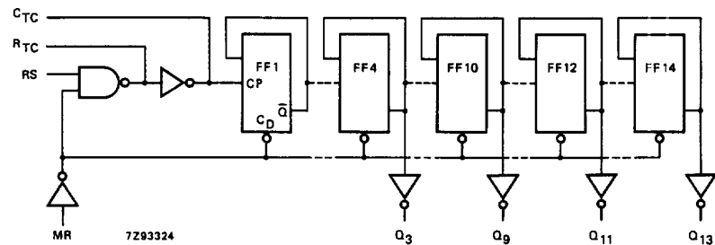
Fig.5 Logic diagram.
