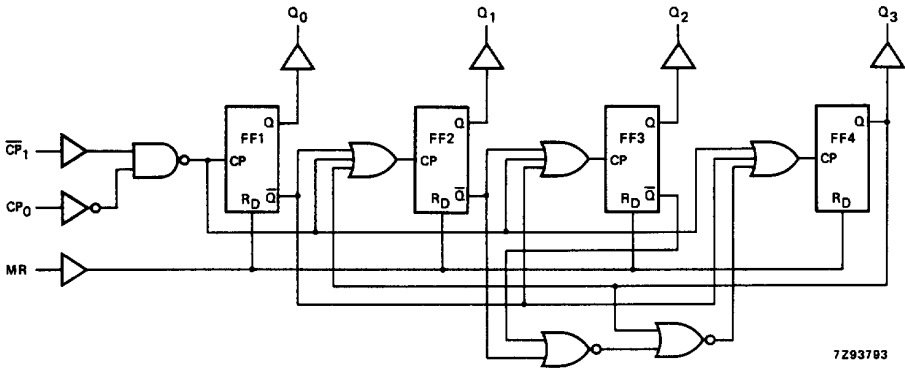
Fig.5 Logic diagram (one counter).
