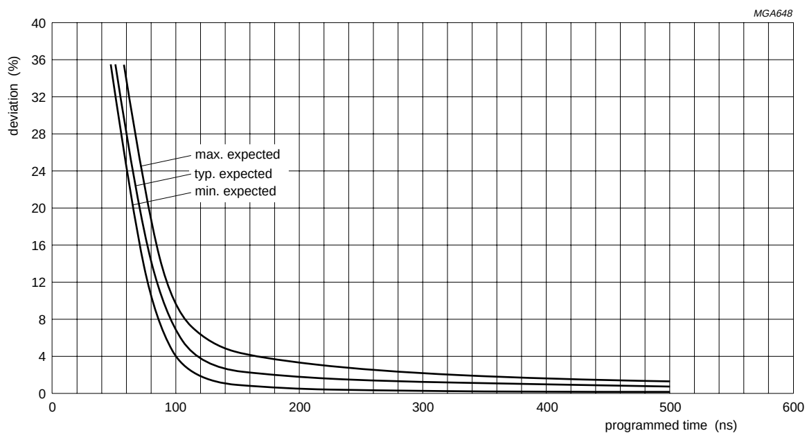
Fig.16 Graphic representation of short time delay accuracy; one stage selected; V_{CC} = 4.5 \text{ V} .
