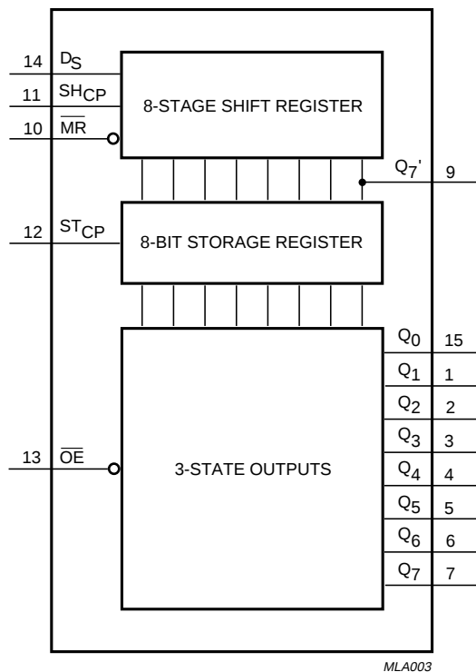
Fig.4 Functional diagram.
