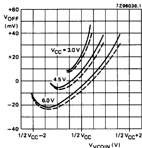
Fig.13 Offset voltage at demodulator output as a function of V_{COIN} and R_S .
