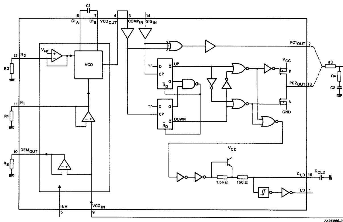
Fig.5 Logic diagram.
