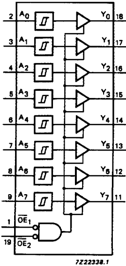
Fig.4 Functional diagram.
