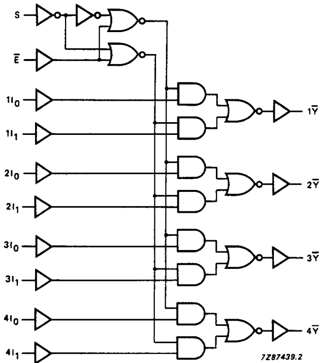
Fig.5 Logic diagram.
