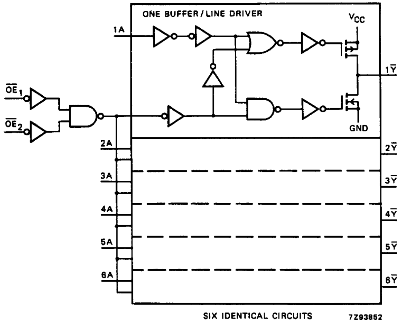
Fig.5 Logic diagram.
