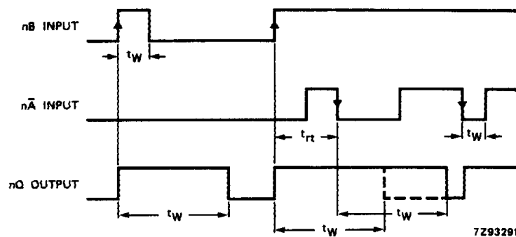
Fig.7 Output pulse control using retrigger pulse; n\bar{R}_D = \text{HIGH} .
