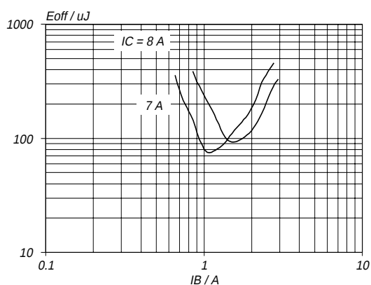
Fig.11. Typical turn-off losses. T_J = 85^\circ\text{C} E_{off} = f(I_B) ; parameter I_C ; f = 32\text{ kHz}
