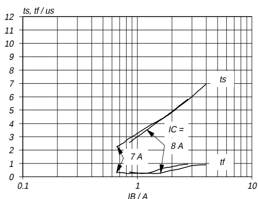
Fig.12. Typical collector storage and fall time. t_s = f(I_B) ; t_f = f(I_B) ; parameter I_C ; T_J = 85^\circ\text{C} ; f = 32\text{ kHz}
