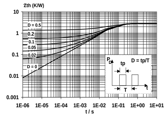
Fig.12. Transient thermal impedance.
