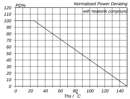
Fig.11. Normalised power dissipation. PD\% = 100 \cdot P_D / P_{D\ 25^\circ C}
