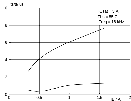
Fig.10. Typical collector storage and fall time. I_{C\text{sat}} = 3\text{ A} ; T_j = 85^\circ\text{C} ; f = 16\text{ kHz}
