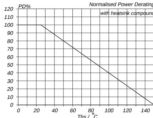
Fig. 12. Normalised power dissipation. PD\% = 100 \cdot P_D / P_{D 25^\circ\text{C}}
