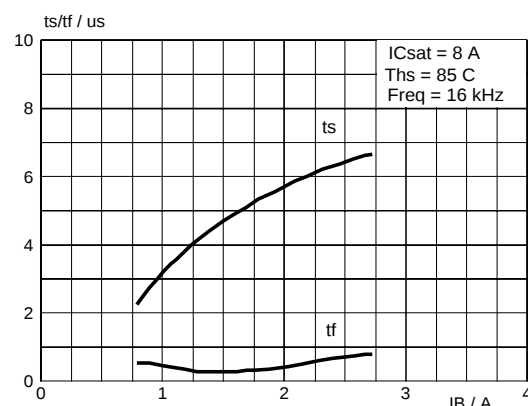
Fig. 11. Typical collector storage and fall time. I_C = 8 \text{ A} ; T_j = 85^\circ\text{C} ; f = 16\text{kHz}
