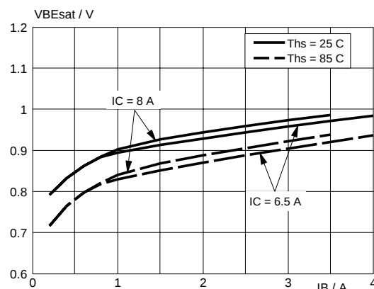
Fig. 10. Typical base-emitter saturation voltage.
