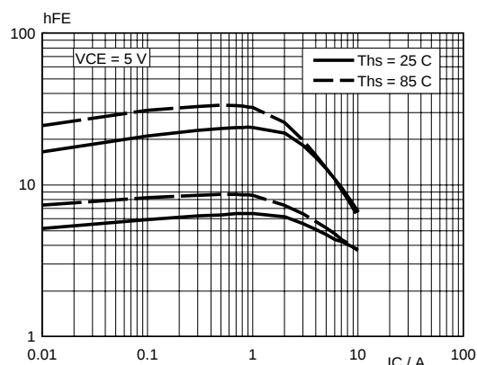
Fig. 8. High and low DC current gain.
