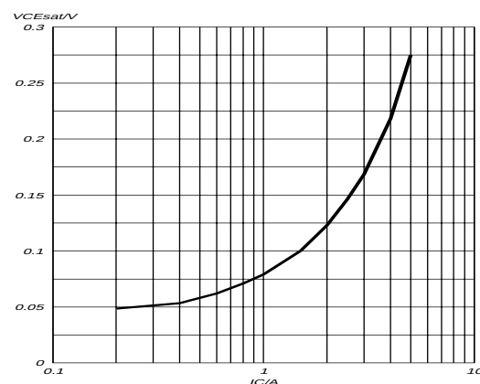
Fig.11. Collector-Emitter saturation voltage. Solid lines = typ values, V_{CEsat} = f(I_C) ; at I_C/I_B = 4 .
