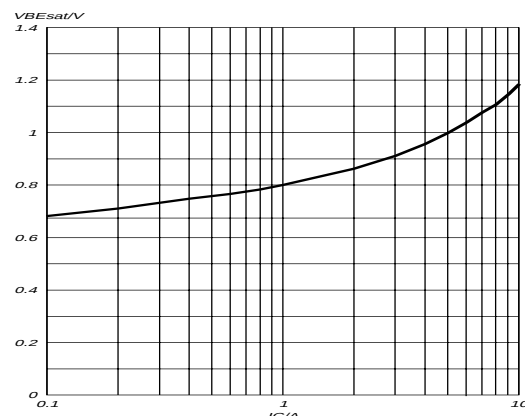
Fig.10. Base-Emitter saturation voltage. Solid lines = typ values, V_{BEsat} = f(I_C) ; at I_C/I_B = 4 .
