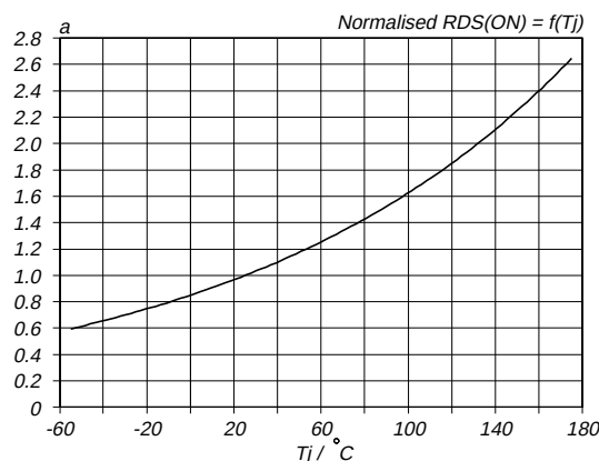
Fig.9. Normalised drain-source on-state resistance. a = R_{DS(ON)} / R_{DS(ON)25\text{ °C}} = f(T_j) ; I_D = 3.5\text{ A} ; V_{GS} = 10\text{ V}
