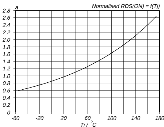
Fig.9. Normalised drain-source on-state resistance. a = R_{DS(ON)} / R_{DS(ON)25\text{ °C}} = f(T_J) ; I_D = 7 A; V_{GS} = 10 V
