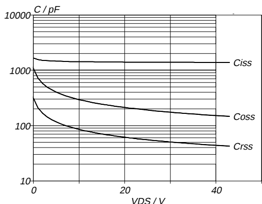
Fig.12. Typical capacitances, C_{iss} , C_{oss} , C_{rss} . C = f(V_{DS}) ; conditions: V_{GS} = 0 V; f = 1 MHz
