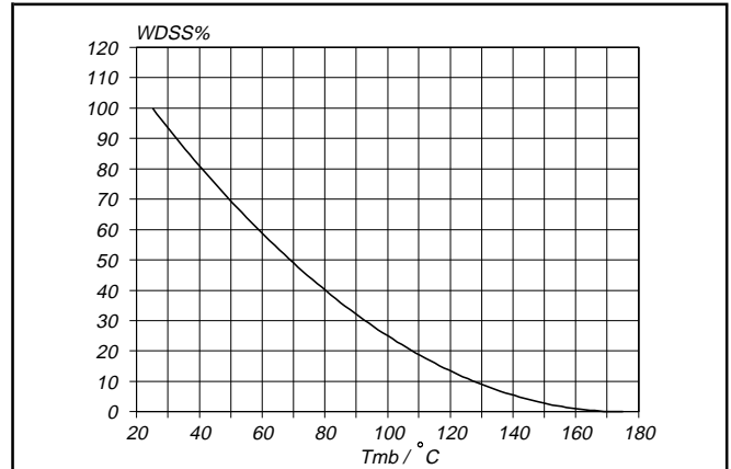
Fig.15. Normalised avalanche energy rating. W_{DSS}\% = f(T_{mb}) ; conditions: I_D = 11 A
