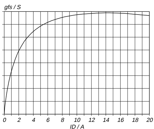
Fig.8. Typical transconductance, T_j = 25 °C. g_{fs} = f(I_D) ; conditions: V_{DS} = 25 V
