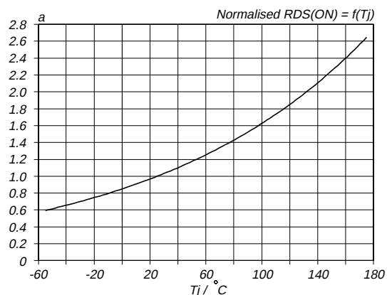
Fig.9. Normalised drain-source on-state resistance. a = R_{DS(ON)}/R_{DS(ON)25\text{ °C}} = f(T_j) ; I_D = 3.5 A; V_{GS} = 5 V
