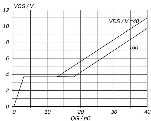
Fig.13. Typical turn-on gate-charge characteristics. V_{GS} = f(Q_G) ; conditions: I_D = 9.2 \text{ A} ; parameter V_{DS}
