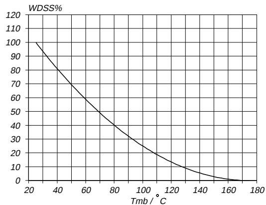
Fig.15. Normalised avalanche energy rating. W_{DSS}\% = f(T_{mb}) ; conditions: I_D = 9 \text{ A}
