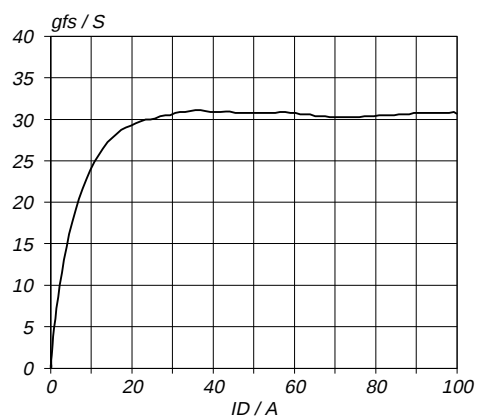
Fig.8. Typical transconductance, T_j = 25 \text{ }^\circ\text{C} . g_{fs} = f(I_D) ; conditions: V_{DS} = 15 \text{ V}
