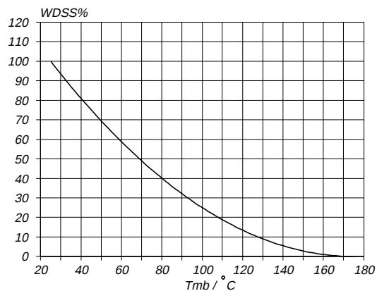
Fig.15. Normalised avalanche energy rating. W_{DSS}\% = f(T_{mb}) ; conditions: I_D = 50 A
