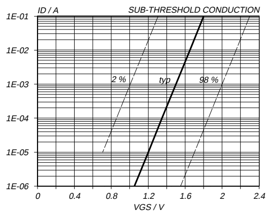
Fig.11. Sub-threshold drain current. I_D = f(V_{GS}) ; conditions: T_j = 25 \text{ }^\circ\text{C} ; V_{DS} = V_{GS}
