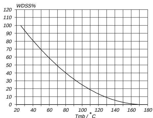
Fig.15. Normalised avalanche energy rating. W_{DSS}\% = f(T_{mb}) ; conditions: I_D = 13 A
