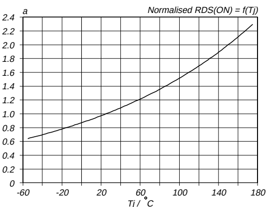
Fig. 9. Normalised drain-source on-state resistance. a = R_{DS(ON)}/R_{DS(ON)25^\circ C} = f(T_j) ; I_D = 6.5 A; V_{GS} = 5 V
