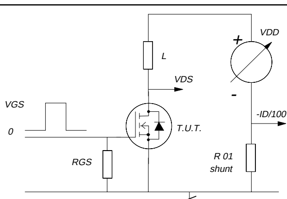
Fig.16. Avalanche energy test circuit.
