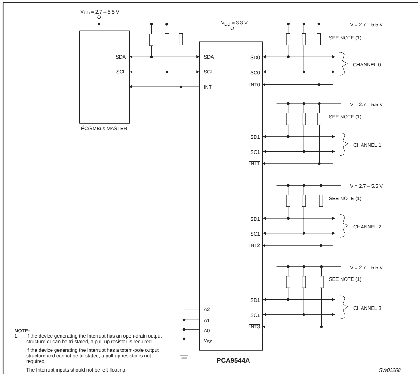
Figure 13. Typical application
