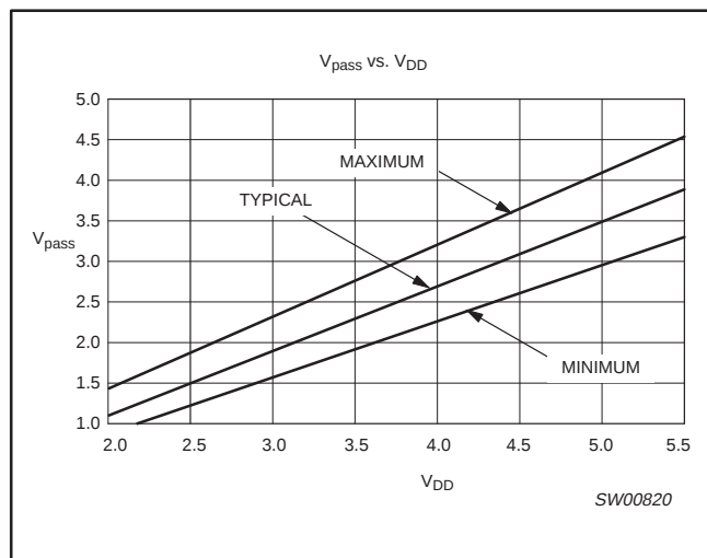
Figure 6. V_{pass} voltage
