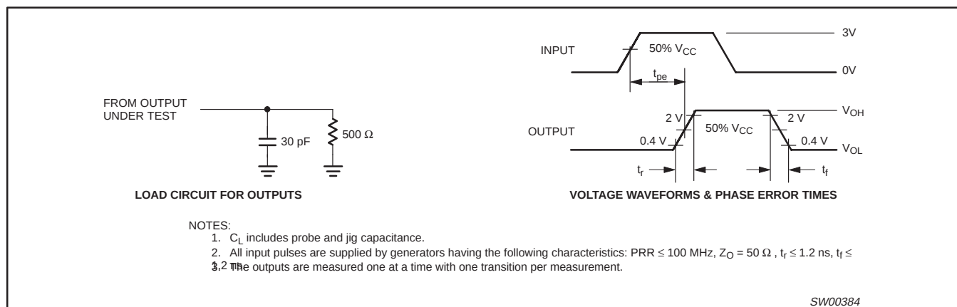
Figure 6. Load Circuit and Voltage Waveforms
