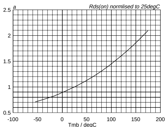
Fig. 9. Normalised drain-source on-state resistance. a = R_{DS(ON)}/R_{DS(ON)25\text{ °C}} = f(T_j) ; I_D = 20\text{ A} ; V_{GS} = 5\text{ V}
